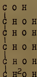
Glucose
